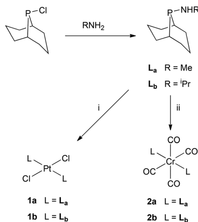
Scheme 2 Reagents: (i) [\text{PtCl}_2(\text{NC}^i\text{Bu})_2] in \text{CH}_2\text{Cl}_2 ; (ii) [\text{Cr}(\text{CO})_4(\text{nbd})] ( \text{nbd} = \text{norbornadiene} ) in \text{CH}_2\text{Cl}_2 .
