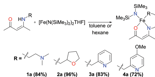
Scheme 2 Synthesis of 1a–4a .
