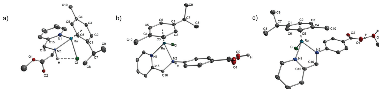
Fig. 2 Molecular structures of complexes 4^+ (a) (only the R_{Ru}, R_N isomer is shown), 5^+ (b) (only the R_{Ru}, R_{N2} isomer is shown; [\text{Ru}_2\text{Cl}_3(p\text{-cym})_2]^+ ( 1^+ ) not shown) and 6^+ (c) (only the R_{Ru} isomer is shown); hydrogen atoms (other than NH or OH), \text{PF}_6^- anions and MeOH in (b) are omitted for clarity. Ellipsoids are drawn at 30% probability.
