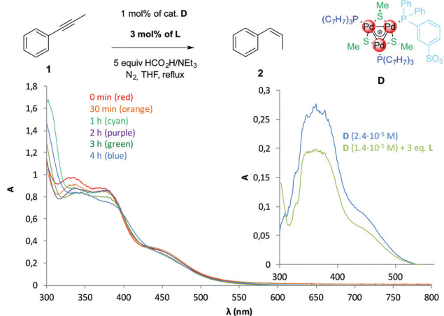
Fig. 3 UV-Vis absorption spectra of samples collected from the catalytic reaction of Table 3, entry 1; 100 μL samples were taken via syringe and diluted with 4.9 mL of degassed THF prior to analyses; the inset presents the absorption spectra of pure D (blue) and D with added tritolyphosphine (green) in THF.
