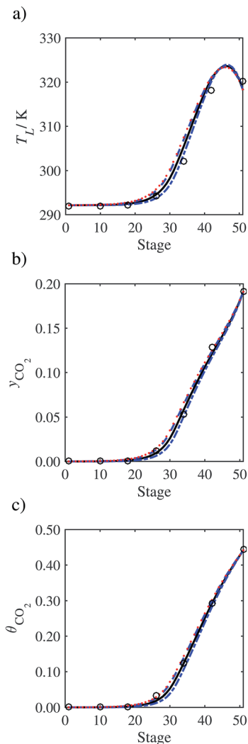
Fig. 22 Sensitivity analysis of the vapour–liquid surface tension on the profiles predicted with our model compared with the experimental pilot-plant data of Run T22 of Tontiwachwuthikul et al. : 15 nominal value (continuous curve), 152 +10 mN m -1 (dashed curve), -10 mN m -1 (dot-dashed curve), and the surface tension correlation for the loaded MEA solution obtained from Jayarathna et al. 153 (dotted curve). (a) Temperature profile for the liquid phase, (b) gas-phase \text{CO}_2 concentration profile, and (c) liquid-phase \text{CO}_2 loading.
