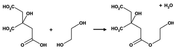
Scheme 5 The transesterification reaction that occurs between citric acid and ethylene glycol in the Pechini process.
