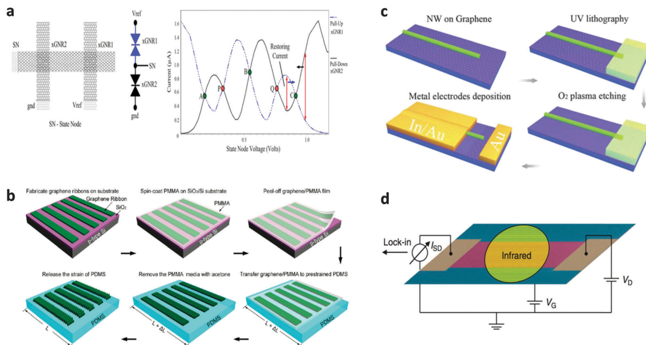
Fig. 17 Application of GNRs. (a) Application of GNRs in cross-bar shaped arrays. (Reproduced with permission from ref. 165, Copyright 2014, Elsevier.) (b) Process for fabricating ripple graphene ribbons for use in strain sensors. (Reproduced with permission from ref. 166, Copyright 2011, The American Chemical Society.) (c) Schematic of the fabrication of a GNR/SNW heterojunction LED. (Reproduced with permission from ref. 180, Copyright 2011, The Royal Society of Chemistry.) (d) Schematic illustration of an IR detector based on GNRs. (Reproduced with permission from ref. 186, Copyright 2013, Nature Publishing Group.)
