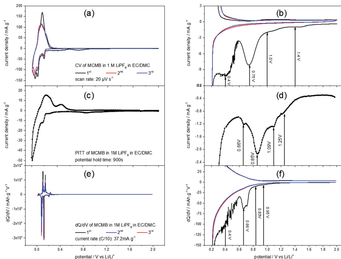
Fig. 2 Voltammograms of MCMB in 1 M \text{LiPF}_6 in EC/DMC (1 : 1) measured by (a and b) cyclic voltammetry (potential sweep rate: 20 \mu\text{V s}^{-1} ) and by (c and d) the potentiostatic intermittent titration technique. For the latter method, the potential was stepwise changed from 2.0 V to 0.01 V and back to 2.0 V in 10 mV steps. After each potential step a current transient was measured for 15 minutes, followed by 15 minutes rest at OCP. The PITT-diagram shows the current density of every transient recorded after 15 minutes at the respective potential. The voltammogram in (e) was derived from a dQ/dV -plot of a charge/discharge curve at a current density of 0.372 \text{ mA g}^{-1} (C/10). (b), (d) and (f) show the magnifications of the CV, PITT and dQ/dV -plot, respectively, in the SEI-formation regime.
