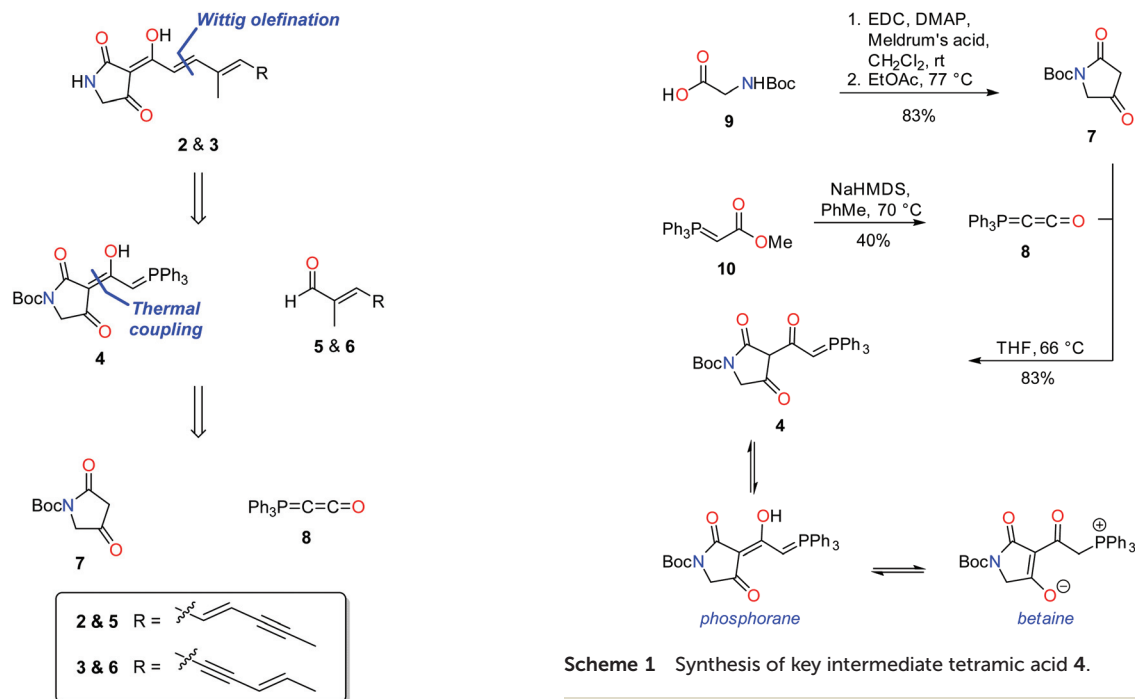
Fig. 2 Retrosynthetic pathway for putative co-metabolites 2 and 3.
