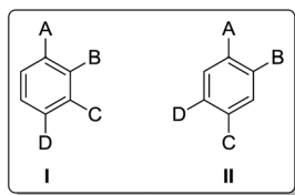
Fig. 3 Tetrasubstituted aromatic building blocks.
