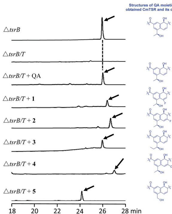
Fig. 2 HPLC analysis of the fermentation cultures of the single mutant strain \Delta tsrB , and double mutant strain \Delta tsrB/T , in the absence or presence of the exogenous QA and its analogs, and the resulting CmTSR products are indicated by the arrows respectively.
