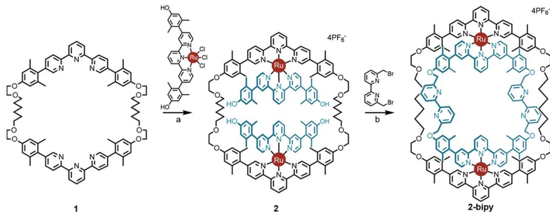
Scheme 2 Synthesis of ring-in-ring structure 2-bipy via the doubly threaded Ring I intermediate 2 . Reaction conditions: (a) 2 : 1 : 1 \text{CH}_2\text{Cl}_2 : EtOH : ethylene glycol, reflux, 12 h, 65%; (b) \text{Cs}_2\text{CO}_3 , acetonitrile, reflux, 72 h, 49%. 13
