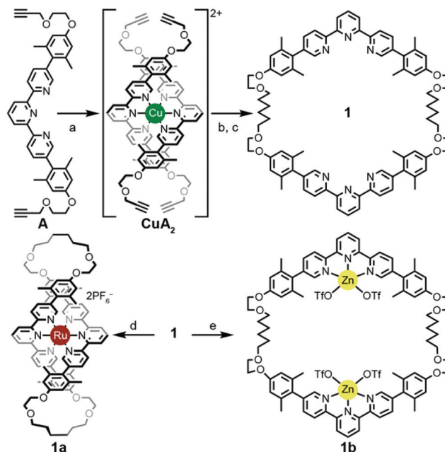
Scheme 3 Synthesis of bis-terpyridine macrocycle 1 and metal complexes 1a and 1b . Reaction conditions: (a) \text{Cu}(\text{OAc})_2 \cdot \text{H}_2\text{O} (0.5 equiv.), ethanol, RT, 1 h; (b) \text{Cu}(\text{OAc})_2 \cdot \text{H}_2\text{O} (10 equiv.), ethanol, reflux, 72 h, 91%; (c) \text{H}_2 , 80 psi, Pd/C (10%), 1:1 ethanol : \text{CH}_2\text{Cl}_2 , 6 h, 91%; (d) \text{Ru}(\text{DMSO})_4\text{Cl}_2 , 10 : 4 : 1 ethylene glycol : dichloroethane : ethanol, reflux, 16 h, 96%; (e) \text{Zn}(\text{OTf})_2 , 1 : 1 ethanol : \text{CH}_2\text{Cl}_2 , RT, 6 h, 97%.
