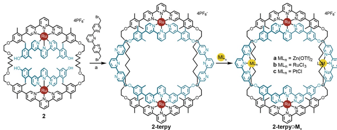
Scheme 4 Synthesis of new ring-in-ring structure 2-terpy and the subsequent coordination of metal ions to give tetrametallic two-ring structures 2-terpy \supset Ma–c . Reaction conditions: (a) \text{Cs}_2\text{CO}_3 , dimethylformamide, reflux, 4 h, 56%; (b) \text{Zn}(\text{OTf})_2 , acetonitrile, RT, 3 h, 94%; (c) \text{RuCl}_3 \cdot 3\text{H}_2\text{O} , 1 : 1 ethanol : 1,2-dichloroethane, 80 °C, 16 h, 99%; (d) \text{PtCl}_2(\text{COD}) , \text{AgBF}_4 , acetonitrile, RT, 30 min, 70%.
