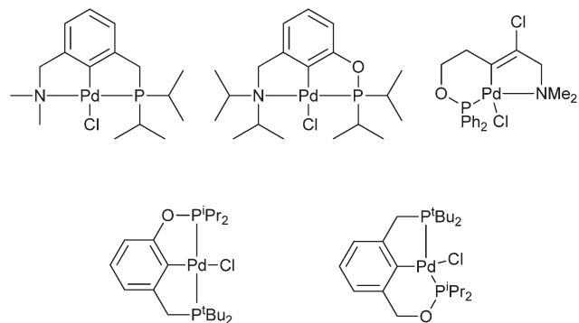
Fig. 3 Unsymmetrical PCN, and P'CP pincer palladacycles.
