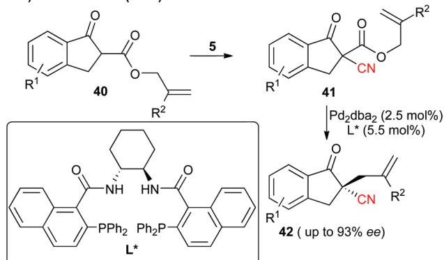
Scheme 7 CBX ( 5 )-mediated \alpha -cyanation reactions of \beta -ketoesters.
