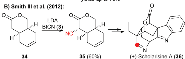
Scheme 5 BtCN-mediated \alpha -cyanation reactions of enolates.
