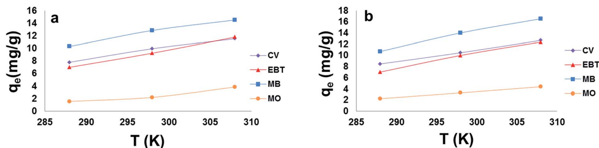
Fig. 10 Effect of temperature on the adsorption capacity ( q_e ) of model dyes onto; [a] MSP NPs and [b] MP NPs. Adsorbent: 5 \text{ g L}^{-1} , dyes 10 \text{ mg L}^{-1} , pH: 2.0 for anionic dyes and 8.0 for cationic dyes, time: 120 min. Magnetite/Pectin Nanoparticles: MP NPs and Magnetite/Silica/Pectin Nanoparticles: MSP NPs.
