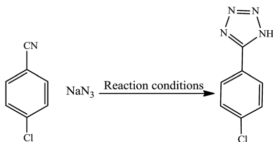
Scheme 2 Preparation of 5-(4-chlorophenyl)-1H-tetrazole.
