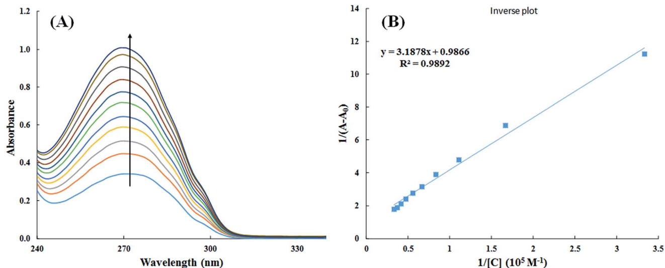
Fig. 9 UV-visible absorption spectra of HSA in absence and presence of varying concentration of cinnamic acid (A) and plot of 1/(A - A_0) vs. 1/[C] (B).
