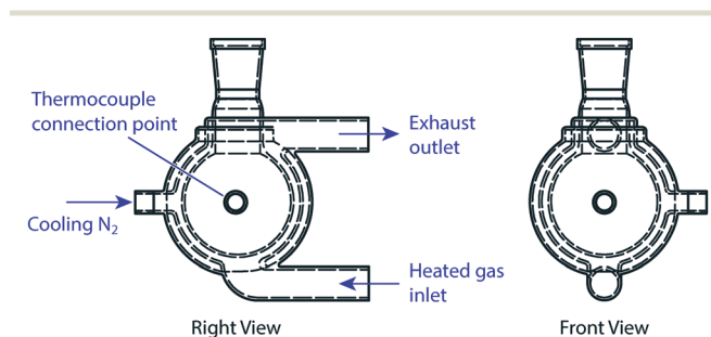
Fig. 4 Schematic for the new glassware that was designed to support batch reactions on the R4+ reactor unit. This study uses two flask sizes: 50 mL and 100 mL.
