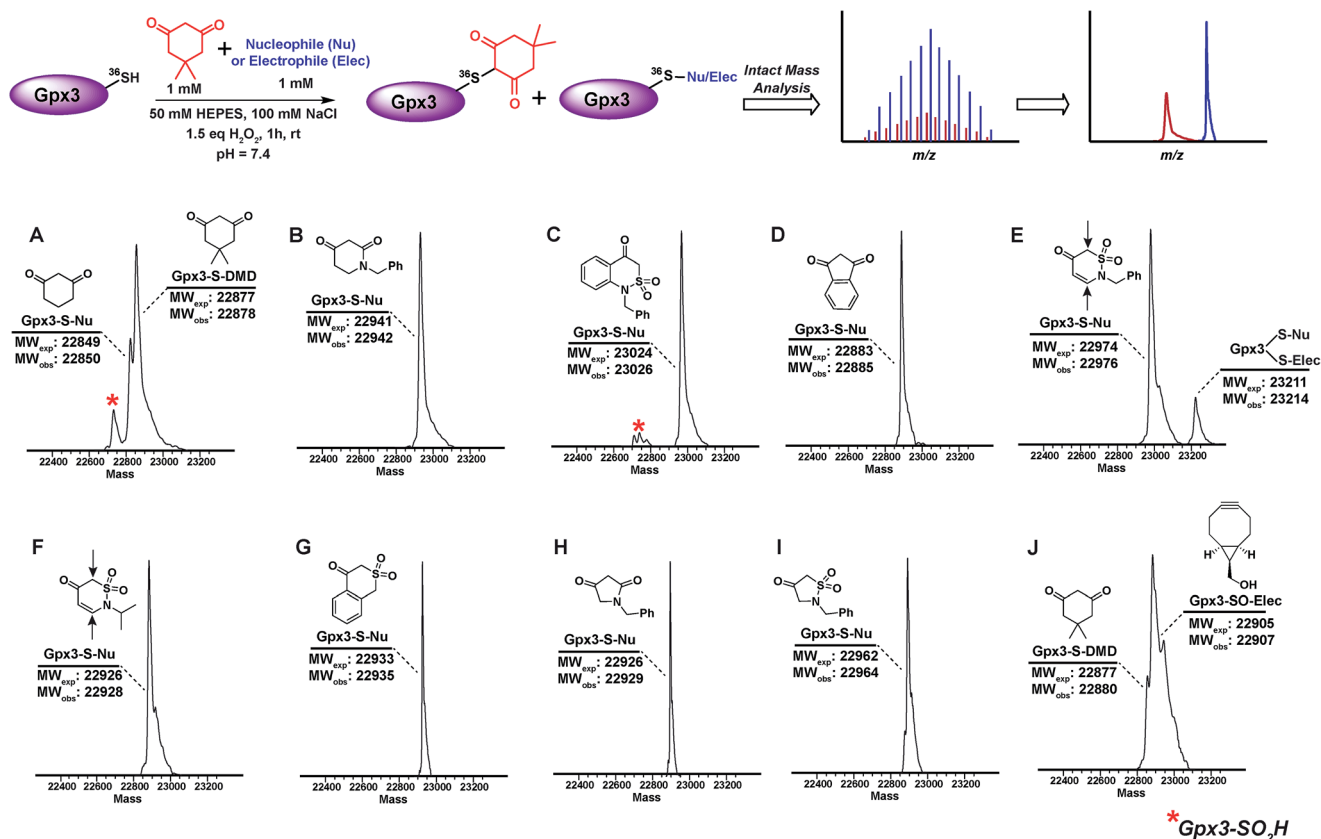
Fig. 3 Competitive labeling of Gpx3-SOH with various nucleophiles in presence of 1 mM dimedone–Gpx3-SH (10 \mu\text{M} ) was incubated with various nucleophiles (1 mM concentration) in presence of dimedone ( 1 ) (1 mM) under oxidizing (1.5 eq. \text{H}_2\text{O}_2 ) conditions. Each sample was analyzed by LTQ-MS for competitive labeling. (A) 1,3-Cyclohexanedione 22a ; (B) 1-benzylpiperidine-2,4-dione 26f ; (C) 1-benzyl-1 H -benzo[ c ] [1,2]thiazin-4(3 H )-one 2,2-dioxide 31h ; (D) 1,3-indandione 34b ; (E) 2-benzyl-2 H -1,2-thiazin-5(6 H )-one 1,1-dioxide 31f ; (F) 2-isopropyl-2 H -1,2-thiazin-5(6 H )-one 1,1-dioxide 31e ; (G) isothiochroman-4-one 2,2-dioxide 31b ; (H) 1-benzylpyrrolidine-2,4-dione 32c ; (I) 2-benzylisothiazolidin-4-one 1,1-dioxide 33f ; (J) ((1 R ,8 S ,9 S )-bicyclo[6.1.0]non-4-yn-9-yl)methanol 5 .
