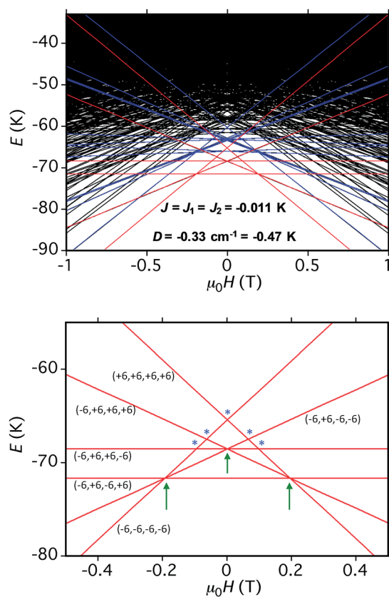
Fig. 14 (Top) simulation with J = -0.0076 \text{ cm}^{-1} ( J/k_B = -0.011 \text{ K} ), ( H = -2J\hat{S}_i \cdot \hat{S}_j convention) and D = -0.33 \text{ cm}^{-1} of the spin state energies vs. applied dc field for an [\text{Mn}_3]_4 tetramer of S = 6 SMMs using eqn (15): red = spin states involving only the m_S = \pm 6 states of the four \text{Mn}_3 sub-units; blue = spin states involving both m_S = \pm 6 states and one m_S = \pm 5 state; black = other states. (Bottom) spin states involving only the m_S = \pm 6 states and their identity. * = multiple spin flips (2, 3 or 4) at the same time. The green arrows are the avoided level crossings at which QTM leads to the three steps at 0.001 \text{ T s}^{-1} in Fig. 11.
