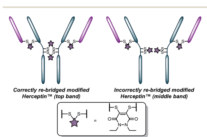
SDS-Page gel of Herceptin™ and use of pyridazinediones 3 & 5:
