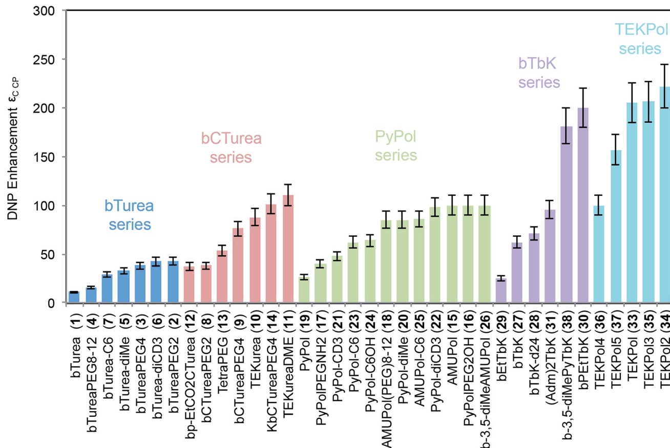
Fig. 2 ^1\text{H} - ^{13}\text{C} CP DNP enhancement ( \epsilon_{CP} ) for bulk solutions of TCE with 16 mM radical.
