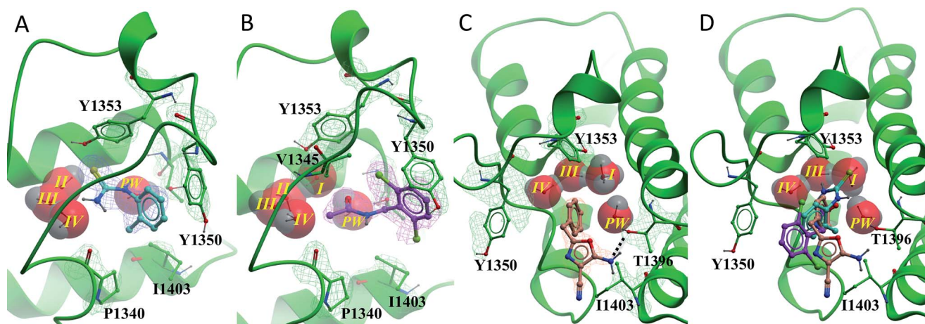
Fig. 5 PHIP(2) (green sticks, ribbons and mesh (2Fo-Fc)) in complex with fragment hits. (A) Thiourea 1 (cyan sticks and mesh (2Fo-Fc)) displaces water I . (B) N -Benzylacetamide 2 (purple sticks and mesh (2Fo-Fc)) binds with all water molecules intact and forms an edge–face interaction with Y1350. (C) Oxazole 3 (cyan sticks and mesh (2Fo-Fc)) forms H-bonds to PW (black dashed line). PHIP(2) orientation has been changed for clarity. (D) Overlay of compounds 1–3 in PHIP(2). In (C) and (D) water II is hidden behind water I .
