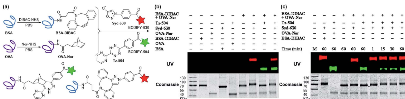
Fig. 3 Modifications of protein surfaces via bioorthogonal cycloadditions. (a) Dibenzocyclooctyne (DIBAC) and 5-norbornene-2-acetic acid (Nor) were appended to BSA and OVA (20 mg mL -1 in PBS) respectively, via NHS ester-amine coupling conditions (20 mM labeling reagent). The labeled proteins BSA-DIBAC and OVA-Nor (2 mg mL -1 ) simultaneously react with sydnone-BODIPY (Syd-630) and tetrazine-BODIPY (Tz-504). (b) Gel analysis of BSA functionalized with DIBAC and OVA functionalized with Nor incubated for 1 h with either Syd-630, Tz-504, both reagents simultaneously, or no reagent (–). (c) Gel analysis of DIBAC-modified BSA and Nor-modified OVA with both Syd-630 and Tz-504 simultaneously for 1–60 min or no reagent (–). The protein loading on the gels was assessed with Coomassie stain.
