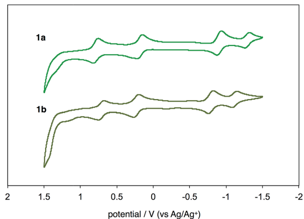
Fig. 7 Cyclic voltammograms of 1a and 1b in CH 2 Cl 2 with n -Bu 4 + N + (CF 3 SO 2 ) 2 N - as supporting electrolyte, and scan rate of 0.1 V s -1 .
