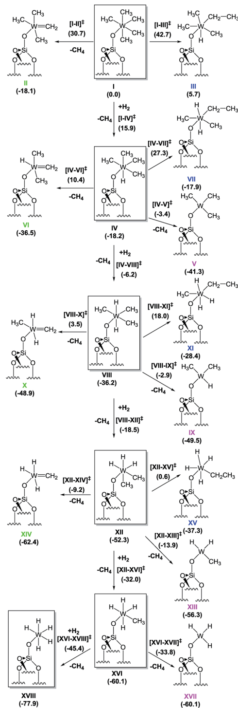
Scheme 2 Proposed mechanism for hydrogenolysis of 1 (i.e., I ) into various tungsten hydrides; the values shown are free energies, in \text{kcal mol}^{-1} . The energetically most favourable hydrogenolysis pathway is highlighted by the structures inside the boxes.
