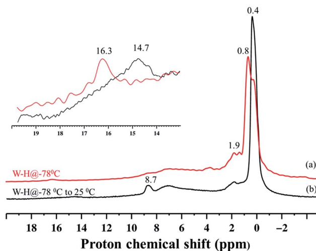
Fig. 5 ^1\text{H} MAS solid-state NMR spectra of fresh 4 (a) and after warming to room temperature and holding for ca. 10 minutes (b). The spectra were acquired at 400\text{ MHz} ( B_0 = 9.4\text{ T} ) with a 10\text{ kHz} MAS frequency, a repetition delay of 5\text{ s} , 8 scans, and at -173\text{ }^\circ\text{C} .
