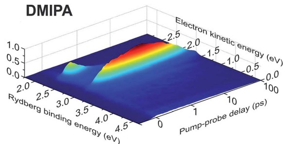
Fig. 4 3D time-dependent photoelectron spectrum of DMIPA obtained using a 200 nm pump/267 nm probe. For clear display of the dynamics over all temporal ranges, the time axis is linear to +1 ps and then logarithmic beyond this point. Full width at half maximum \Delta E/E values for the kinetic energies are \sim 0.1 .
