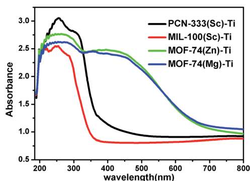
Fig. 4 UV/Vis absorption spectra of PCN-333(Sc)-Ti (black), MIL-100(Sc)-Ti (red), MOF-74(Zn)-Ti (green) and MOF-74(Mg)-Ti (blue).
