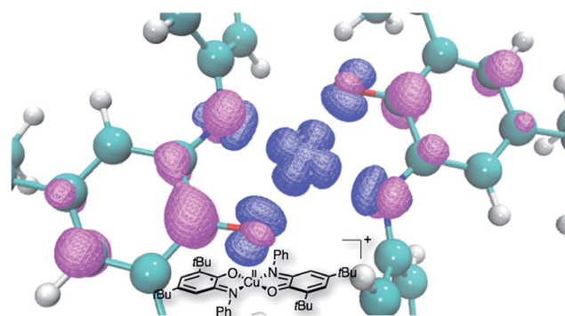
Fig. 3 DFT optimized structure for complex 3 , together with a spin density isosurface (plotted at 0.005\text{e}^- \text{\AA}^{-3} ).
