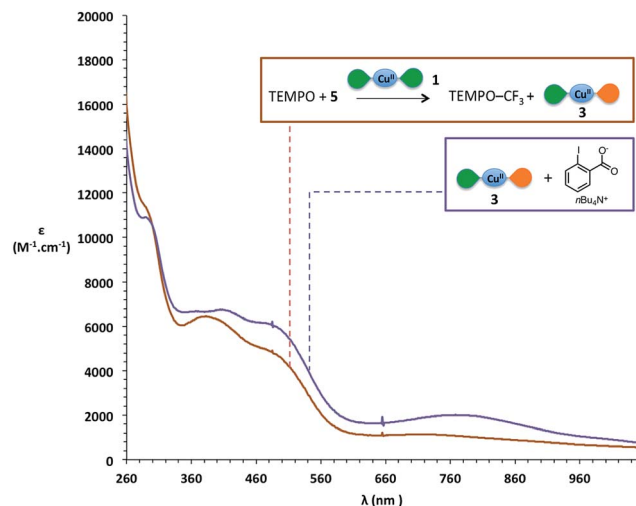
Fig. 5 Comparison of UV-vis spectra in \text{CH}_2\text{Cl}_2 of: brick red: reaction with Togni II's source 5; purple: in situ generated [\text{Cu}(\text{L}^{\text{SQ}})(\text{L}^{\text{BQ}})]^+ \mathbf{3} with added o -iodobenzocarboxylate. Color code for ligands: green petal is SQ ligand and orange petal is BQ ligand.
