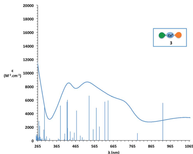
Fig. 4 Comparison of DFT calculated peak positions (blue peaks) and experimental (blue curve) UV-vis spectrum of complex 3.
