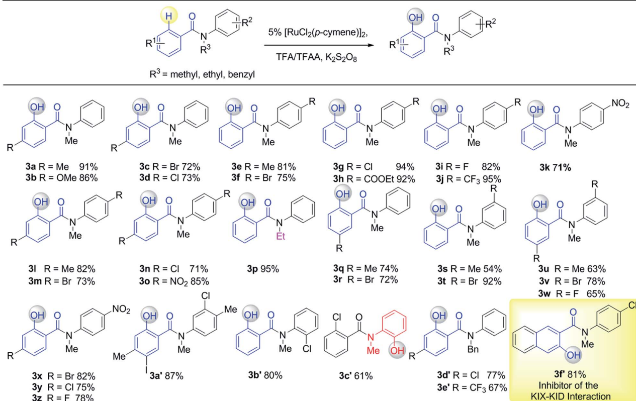
Fig. 2 Substrate scope of Ru(II) in \text{C}(\text{sp}^2)\text{-H} hydroxylation (isolated yield).
