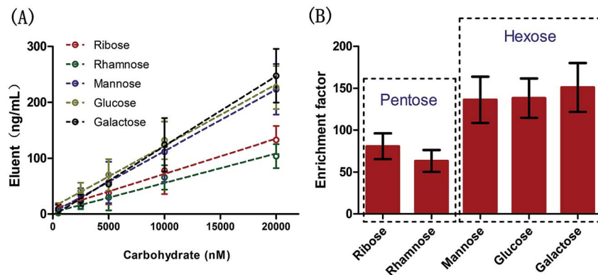
Fig. 5 The linear ranges (A) and enrichment factors (B) of multi-carbohydrates in PBS solution using the proposed probe.
