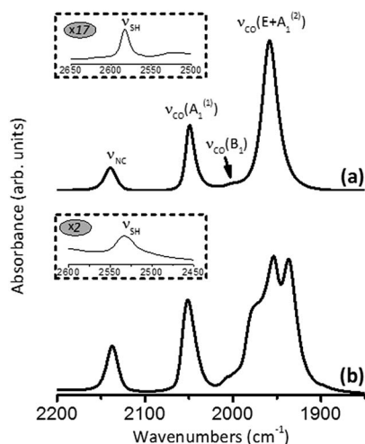
Fig. 12 FTIR spectra of 7 in (a) CH_2Cl_2 and (b) KBr.
