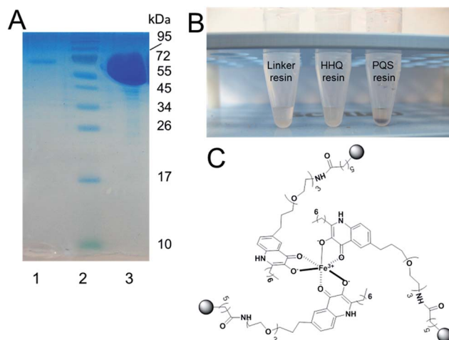
Fig. 1 The PQS affinity probe retains affinity for PqsRLBD and Fe 3 + . (A) Purified PqsR ligand binding domain (PqsRLBD) binds strongly to immobilized PQS but not to the control linker resin. Purified MBP-tagged PqsRLBD was incubated with aliquots of the control or PQS-derivatized resin, see ESI.† The resin samples were extensively washed and the bound protein was eluted by boiling the washed beads in SDS sample buffer. The panel shows a Coomassie Brilliant Blue-stained SDS-PAGE gel of the protein eluting from control beads (lane 1) or PQS-derivatized beads (lane 3). Molecular mass markers are shown in lane 2. (B) Aliquots (50 μL) of control beads, HHQ beads or PQS beads (as indicated) were mixed with 1 mM FeCl 3 . The PQS beads immediately turned deep red due to the formation of the PQS-iron complex. (C) Proposed structure of the PQS-Fe complex on probe resulting in dark red colouration.
