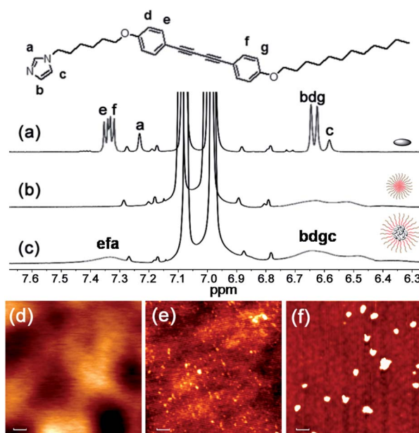
Fig. 2 Characterizations of P-M : partial 1 H NMR spectra (400 MHz, room temperature) of (a) M , (b) P and (c) P-M in toluene- d 8 . The tiny peaks without labels are assigned to satellite peaks from the solvent. AFM images of (d) M , (e) P and (f) P-M spun from toluene solution, respectively. Scale bar: 100 nm.
