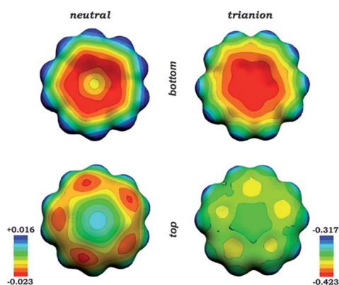
Fig. 4 Molecular electrostatic potentials (MEPs) of the neutral \text{C}_{20}\text{H}_{10} molecule (left) and discrete \text{C}_{20}\text{H}_{10}^{3-} anion (right).
