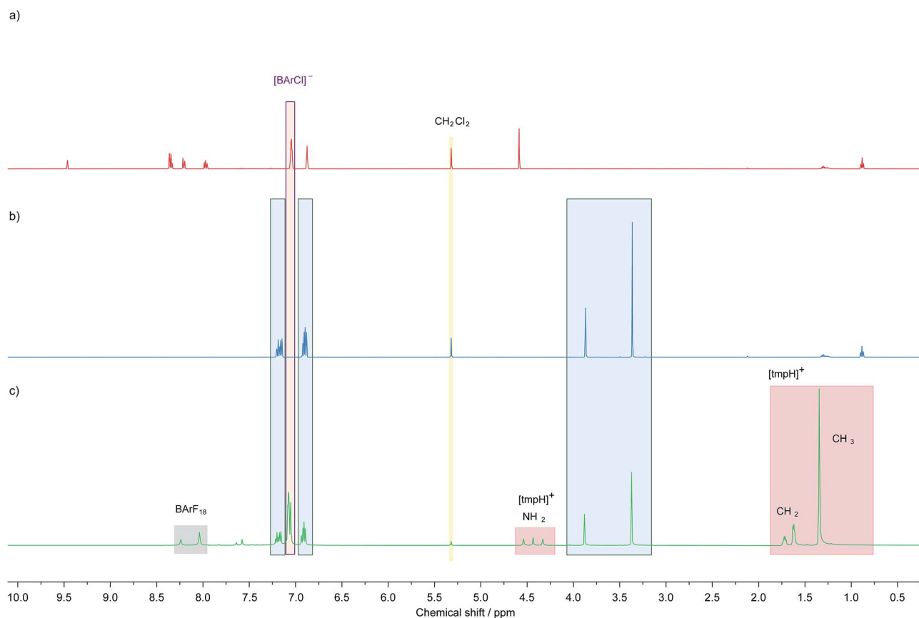
Fig. 2 ^1\text{H} NMR spectra demonstrating the ability of [(\mu\text{-H})(\text{BARF}_{18})_2]^- and [\text{H}-\text{BARF}_{18}]^- to transfer hydride to \mathbf{1}[\text{BARCl}] in \text{CD}_2\text{Cl}_2 , (a) \mathbf{1}[\text{BARCl}] , (b) authentic \mathbf{1}\text{-H} , and (c) an equimolar mixture of \mathbf{1}[\text{BARCl}] and [\text{tmpH}][(\mu\text{-H})(\text{BARF}_{18})_2]^- after 30 minutes at 20 °C.
