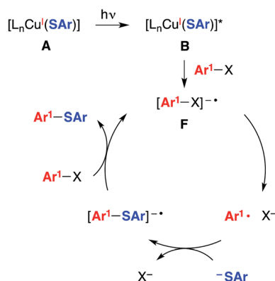
Fig. 3 An alternative mechanism: S RN 1 (radical chain process). 5
