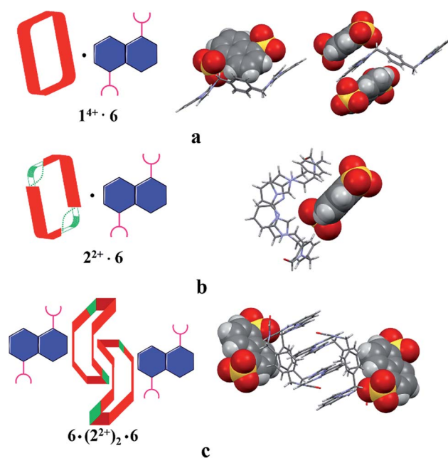
Fig. 5 Schematic views and single crystal X-ray structure of (a) [1^{4+} \cdot 6 \cdot 6H_2O] , [1^{4+} \cdot 6 \cdot 14H_2O]^{22c} , (b) [2^{2+} \cdot 6 \cdot 2.5H_2O] and (c) 6 \cdot (2^{2+})_2 \cdot 6 . Some of the counter ions and solvent molecules have been omitted for clarity.
