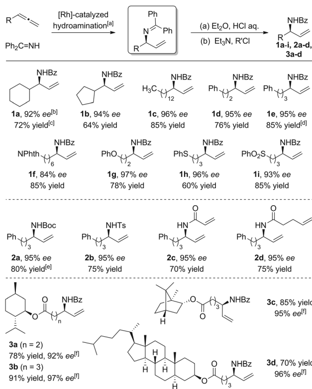
Scheme 3 Scope of allenenes and one-pot synthesis of allylic amides. [a] Benzophenone imine (1.0 equiv., 0.4 mmol), allene (1.5 equiv.), [(Rh(COD)Cl) 2 ] (2.0 mol%), L4 (4.0 mol%), PPTS (20 mol%), DCE (1.0 ml). [b] Determined by chiral HPLC. [c] Yield is that of the isolated product. [d] The reaction was performed in 0.2 mmol scale. [e] Boc 2 O was used in the protection step. Phth = phthaloyl; Ts = 4-methylbenzene-1-sulfonyl. [f] Determined by chiral HPLC after transesterification with ethanol.
