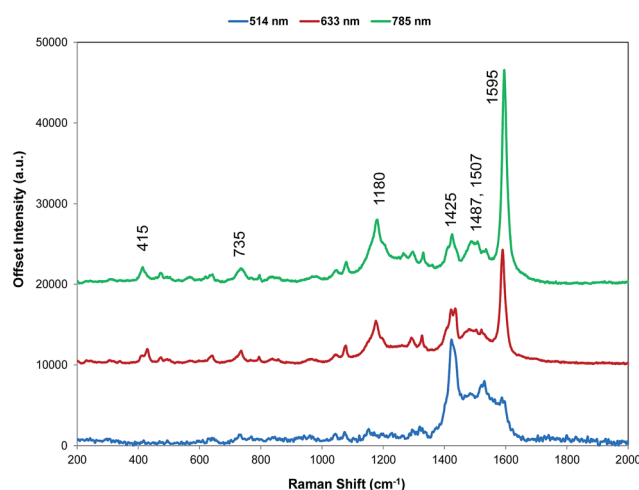
Fig. 2 Resonance Raman spectra for dye 1 at three excitation wavelengths ( 514 , 633 , and 785 \text{ nm} ). The 514 \text{ nm} spectrum is multiplied by a factor of 10 for clarity. The 785 \text{ nm} Raman bands which are discussed throughout have been labelled accordingly but for a detailed interpretation of all peaks, see Table S1, ESI.†
