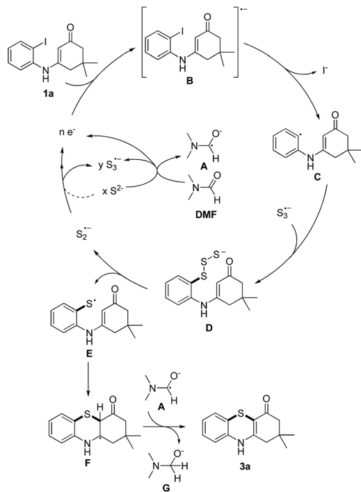
Scheme 4 Plausible mechanism.
