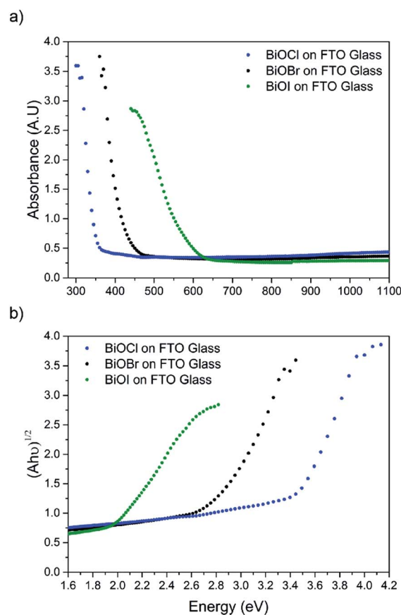
Fig. 5 (a) UV/vis spectra of BiOX ( X = \text{Cl}, \text{Br}, \text{I} ) films deposited on FTO glass and (b) corresponding Tauc plots.
