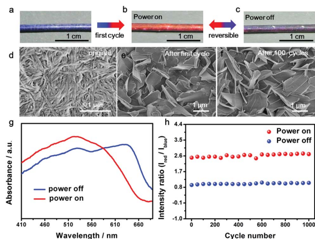
Fig. 2 Electrothermal chromatic behavior of the composite fiber. (a–c) Photographs of the electrothermal chromatic composite fiber in the first power on/off cycle; (b and c) are reversible in the following cycles. (d–f) SEM images of PDA in the composite fiber. PDA formed nanofibers at the original state (d), changed to microsheets after the first power on/off cycle (e) and maintained the morphology of the microsheets after the 100th cycle (f). (g) UV-vis spectra of the composite fiber at the power "off" and "on" states. (h) The intensity ratios of red to blue peaks at the "off" and "on" states for 1000 cycles.
