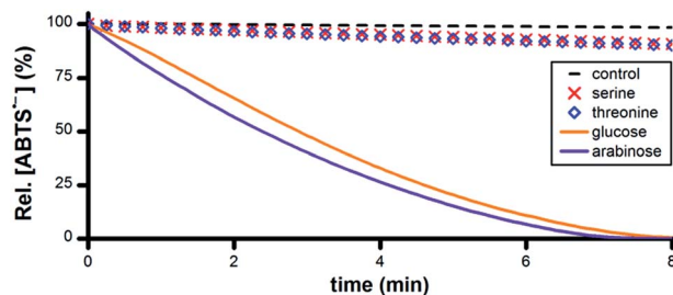
Fig. 5 Plot of relative [\text{ABTS}^{\bullet-}] vs. time following the addition of amino acid or sugar ( t = 0 ) to PBS solutions containing \text{ABTS}^{\bullet-} and Ru1 . Conditions: [\text{Ru1}]_0 = 5 \mu\text{M} , [\text{ABTS}^{\bullet-}]_0 = 50 \mu\text{M} , [\text{ROH}]_0 = 50 \text{mM} , PBS (pH 7.4), 25^\circ\text{C} ; [\text{ABTS}^{\bullet-}] determined using absorbance measured at 734 \text{nm} and \epsilon_{734} = 1.5 \times 10^4 \text{M}^{-1} \text{cm}^{-1} (ref. 33).
