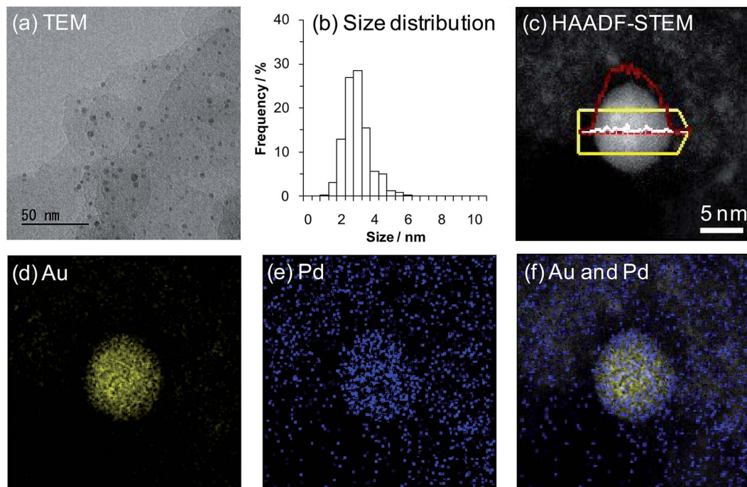
Fig. 1 (a) TEM image of \text{Au}_9\text{Pd}_1/\text{LDH} . (b) The size distribution of \text{Au}_9\text{Pd}_1/\text{LDH} . (c) HAADF-STEM image of \text{Au}_9\text{Pd}_1/\text{LDH} . EDS intensity line profiles are shown in red (Au) and white (Pd) lines. (d) EDS elemental map of Au. (e) EDS elemental map of Pd. (f) Overlap of EDS elemental map of Au and Pd.
