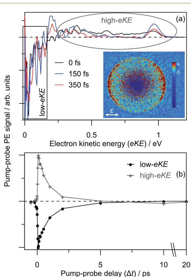
Fig. 8 3.10 + 1.05 eV time-resolved dynamics: (a) three example \Delta t spectra, which are divided into low-eKE and high-eKE contributions; and (b) integrated contributions of each the two pump-probe contributions. The 150 fs pump-probe velocity-map image is inset in (a), illustrating \beta_2 \sim +2 (relative to the polarisation, \epsilon ) for the high-eKE feature.
