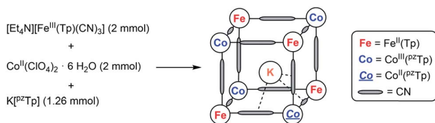
Scheme 1 Simplified synthesis of 1 (further details, see ESI†).
