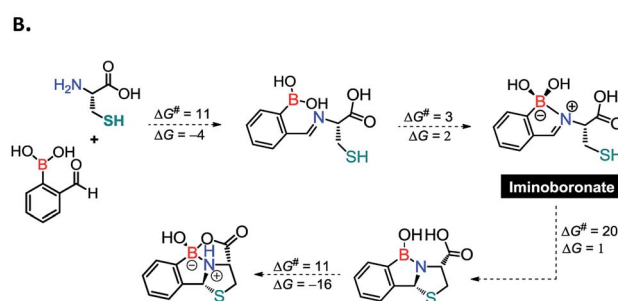
Scheme 4 (A) Difference in stability between the four more stable diastereomers of product 1 . (B) Schematic representation of the most important intermediates in the mechanism of formation of 1 from Cys and 2FBBA. Free energy values in kcal mol -1 .
