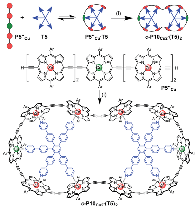
Scheme 3 Synthesis of c\text{-P10Cu}_2\cdot(\text{T5})_2 . Two representations of the synthetic route used to prepare c\text{-P10Cu}_2\cdot(\text{T5})_2 . Reaction conditions: (i) \text{PdCl}_2(\text{PPh}_3)_2 , \text{CuI} , 1,4-benzoquinone, i\text{-Pr}_2\text{NH} , \text{CHCl}_3 , 17%. Ar = 3,5-bis( tert -butyl)phenyl.
