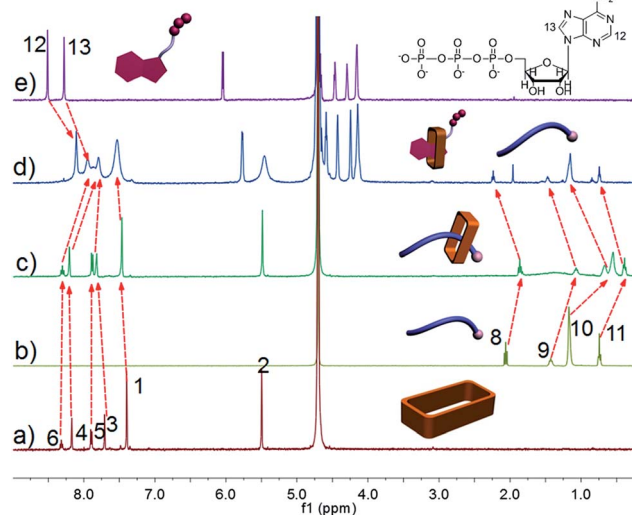
Fig. 7 ^1\text{H} NMR spectra (500 MHz, \text{D}_2\text{O} , 298 K): (a) 3.00 mM 1 ; (b) 3.00 mM 2 ; (c) 1 and 2 (3.00 mM for each); (d) 1 , 2 , and ATP (3.00 mM for each); (e) 3.00 mM ATP.
